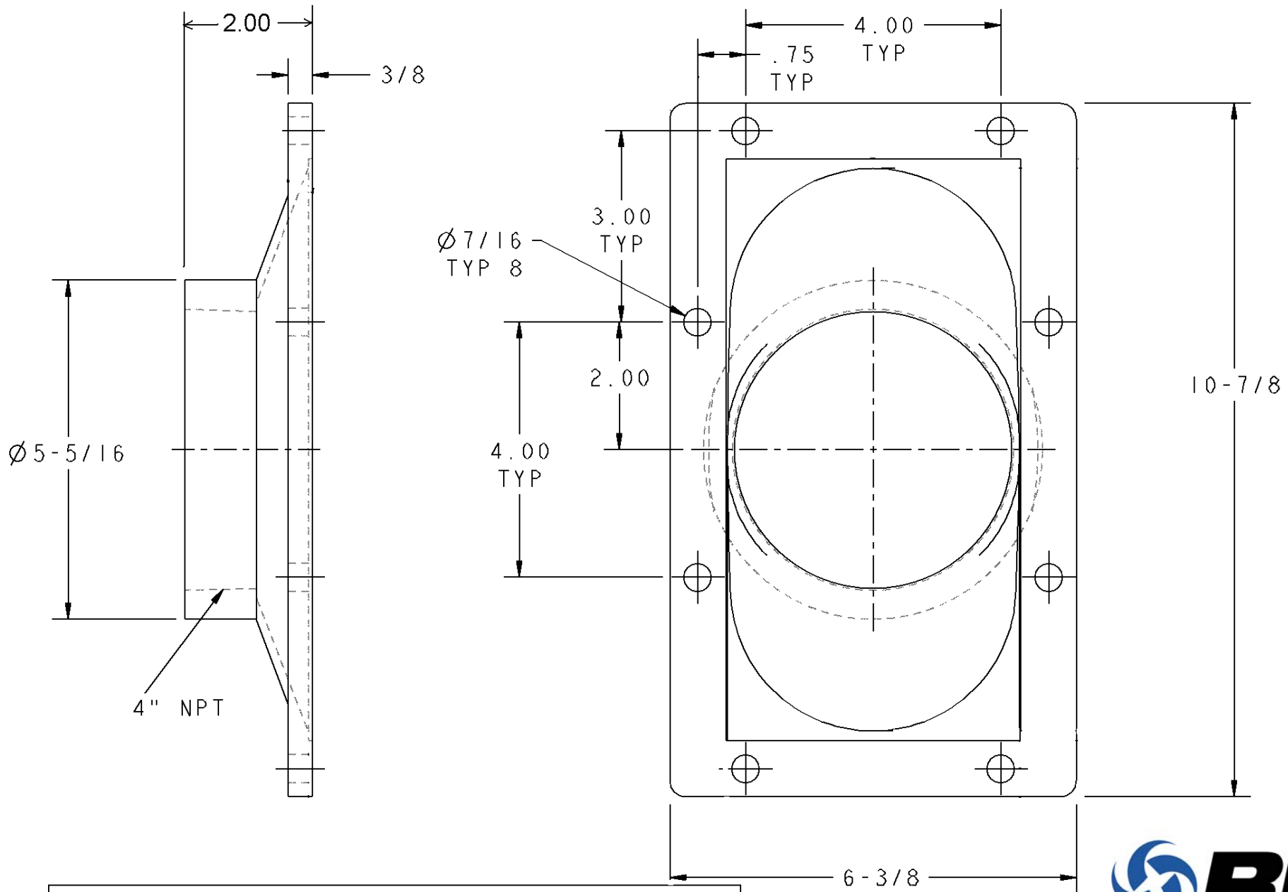
SHORT CONNECTOR, INLET/DISCH 409 ROOTS-FLO
